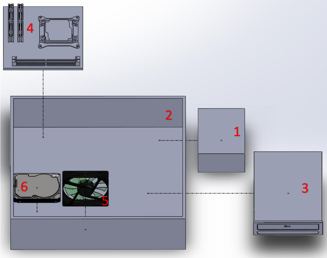
Exploded Diagram 1
