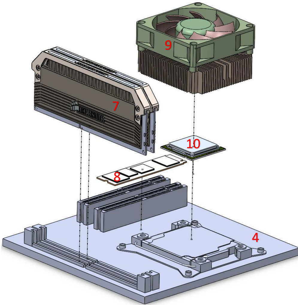
Exploded Diagram 2
