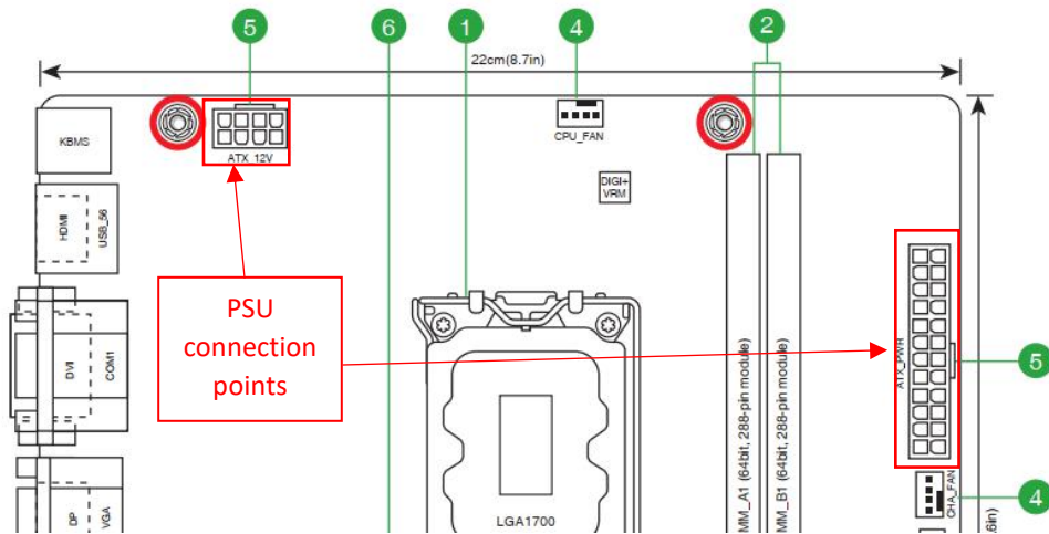
Motherboard Diagram for PSU Connections
