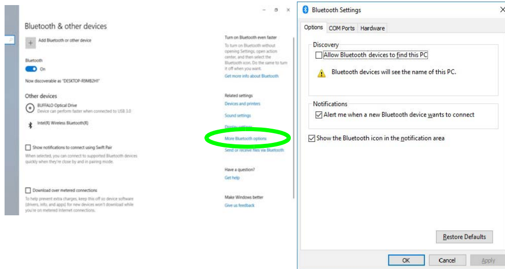
Figure 6 - 14 Bluetooth Settings
