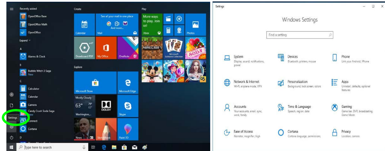
Figure 1 - 18 - Settings
