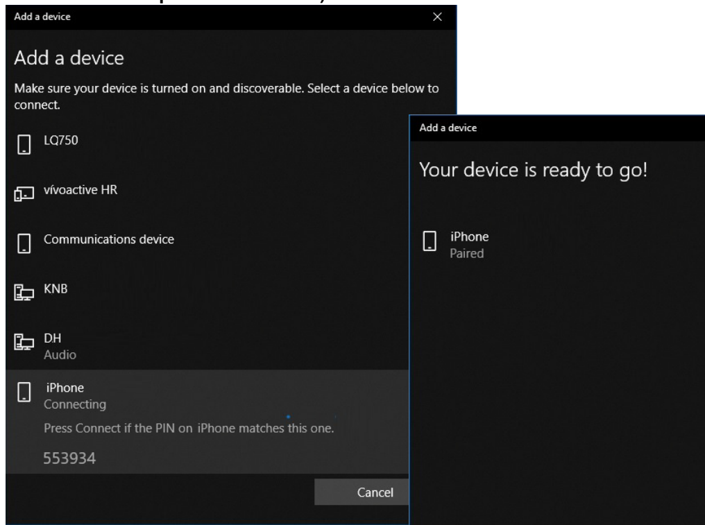
Figure 6 - 12 Bluetooth Connect
