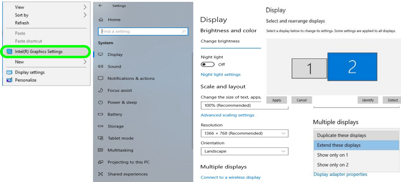
Figure 1 - 22 - Display Settings
