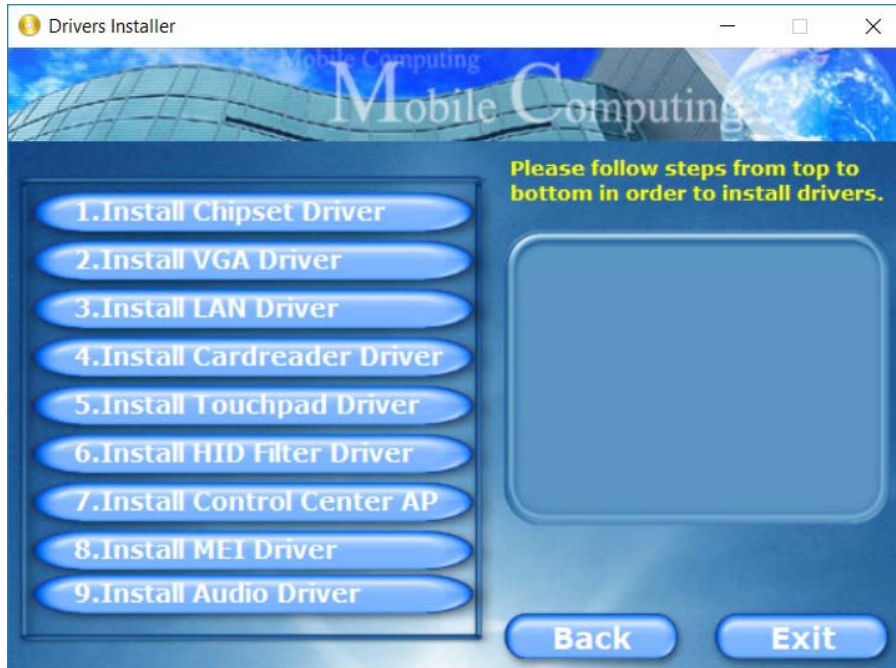
Figure 4 - 2 - Install Drivers
