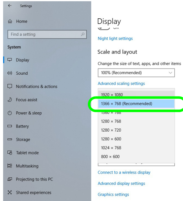
Figure 1 - 24 - Display (Resolution)
