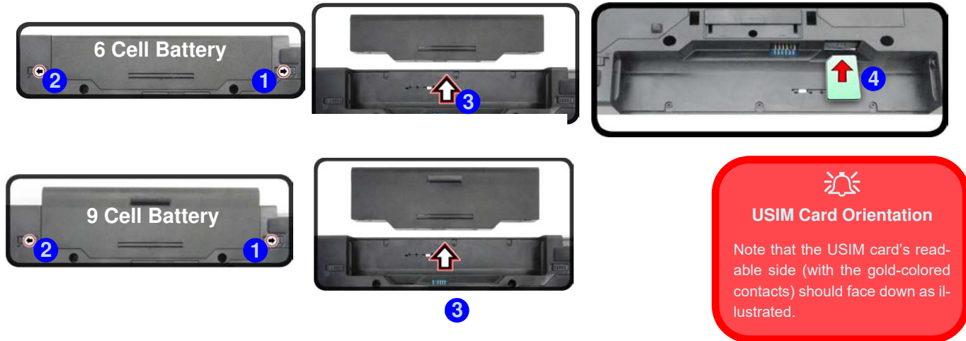
Figure 1 - 10 - Battery Removal & USIM Card Insertion
